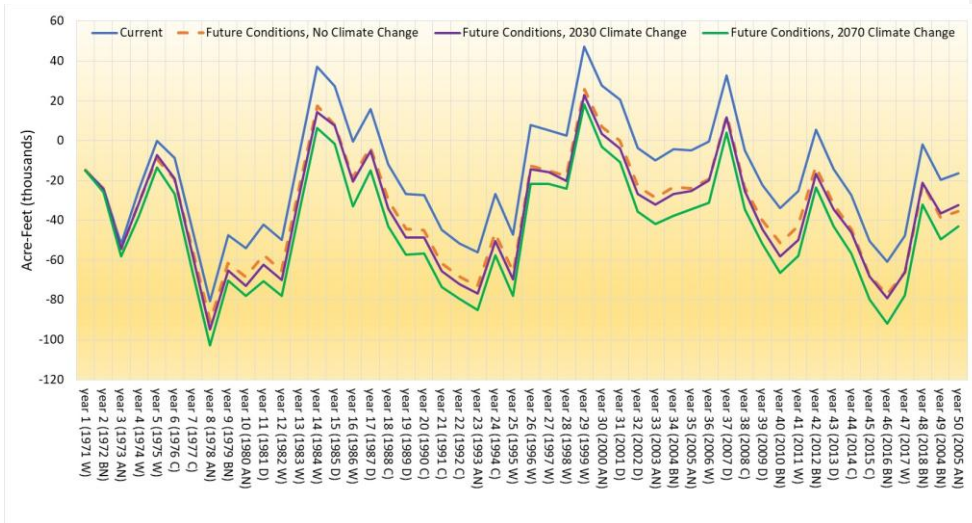
Figure ES-8: Cumulative Change in Groundwater Storage for Current and Future Conditions Baseline Scenarios (BBGM v. 1.0)
