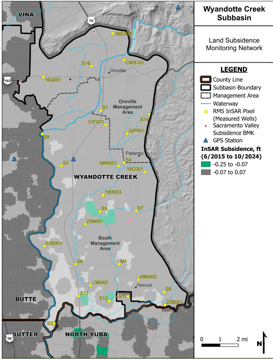
Figure 4-7. Land Subsidence Monitoring Network
