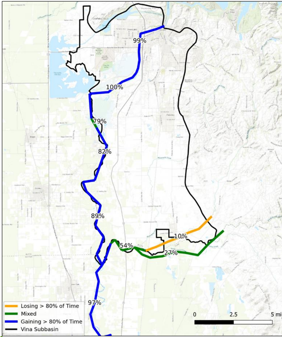
Figure 2-20: Wyandotte Creek Subbasin Gaining and Losing Stream Reaches Based on the BBGM v.1.3, Water Years 2000 to 2024.
