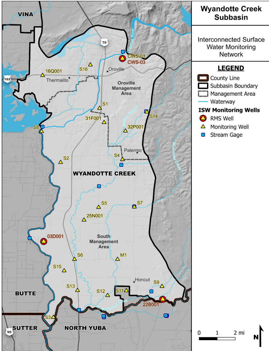
Figure 4-4. Interconnected Surface Water Monitoring Network.
