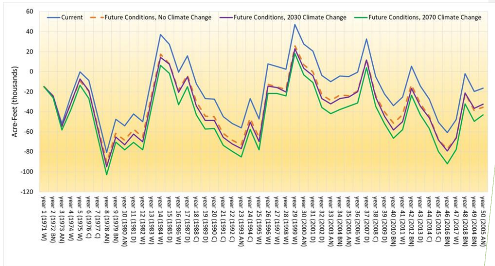
Figure 2-36: Cumulative Change in Groundwater Storage for Current and Future Conditions Baseline Scenarios (BBGM v.1.0)
