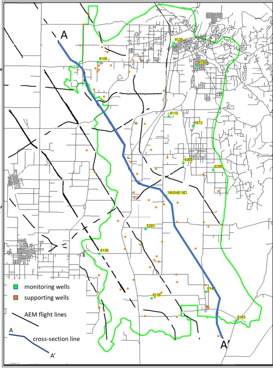
Figure 2-8A. Wyandotte Creek Subbasin AEM Flightlines,
